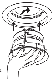
Figure 2 Connect the wires and place the loudspeaker in the frame, twist and lock.
